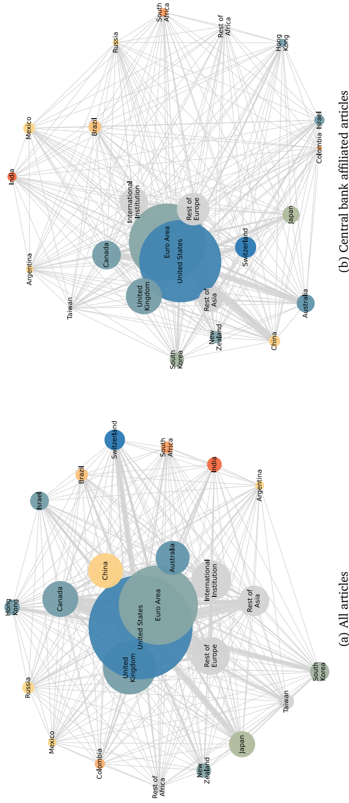
Figure 4: Citation Networks
